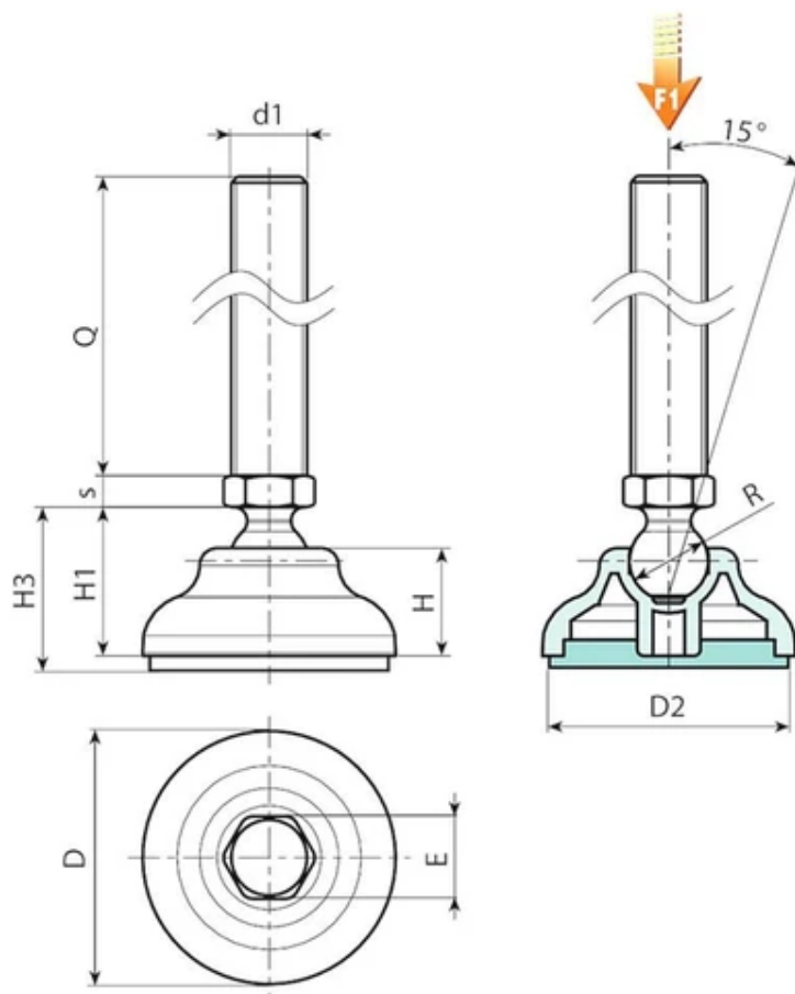
Version P901: Mounting foot with stem type A (with hexagonal base) and ball 12.4 - with SBS non-slip base
